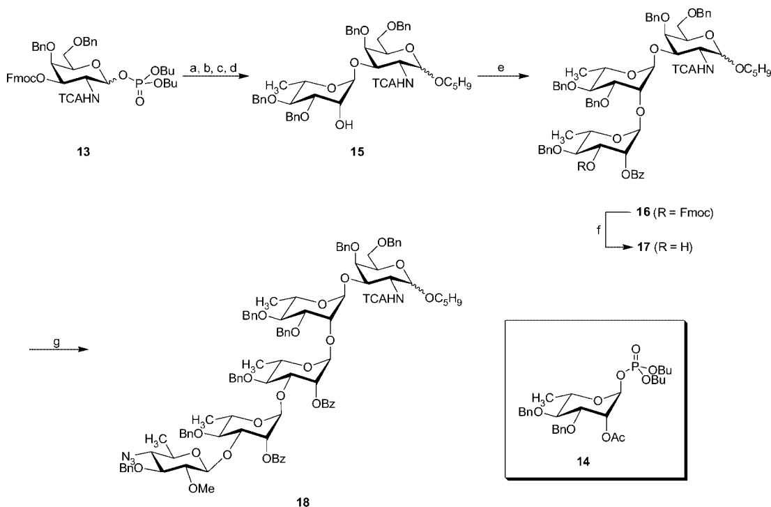
Scheme 3. Assembly of pentasaccharide 18 . Reagents and conditions: a) 4-penten-1-ol, TMSOTf, \text{CH}_2\text{Cl}_2 , 4-Å mol. sieves, -30^\circ\text{C} , 90 min, 70%; b) 20% piperidine in DMF, 25^\circ\text{C} , 1 h, quant.; c) 14 , TMSOTf, \text{CH}_2\text{Cl}_2 , 0^\circ\text{C} , 90 min, 77%; d) NaOMe, MeOH, 25^\circ\text{C} , 12 h, 91%; e) 7 , TMSOTf, \text{CH}_2\text{Cl}_2 , 0^\circ\text{C} , 90 min, 61%; f) \text{NEt}_3 , \text{CH}_2\text{Cl}_2 , 25^\circ\text{C} , 4 h, 89%; g) 12 , TMSOTf, \text{CH}_2\text{Cl}_2 , -2^\circ\text{C} , 90 min, 73%.
