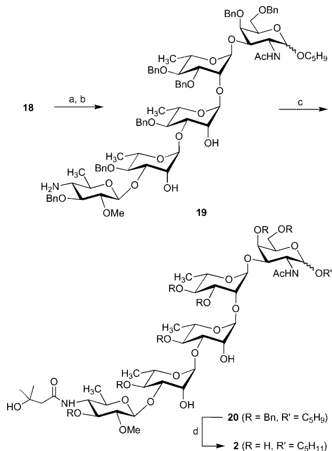
Scheme 4. Completion of the total synthesis of 2 . Reagents and conditions: a) \text{Bu}_3\text{SnH} (excess), AIBN (cat.), toluene, 100^\circ\text{C} , 2 h, 54%; b) \text{NaOMe} , \text{BuNH}_2 (excess), \text{MeOH} , 25^\circ\text{C} , 18 h, 73%; c) 3-hydroxy-3-methylbutanoic acid, HATU, DIPEA, \text{DMF} , 25^\circ\text{C} , 4 h, 44% (after HPLC); d) \text{Pd/C} , \text{MeOH/THF/H}_2\text{O} (4:4:1), \text{H}_2 , 25^\circ\text{C} , 18 h, 63%.
