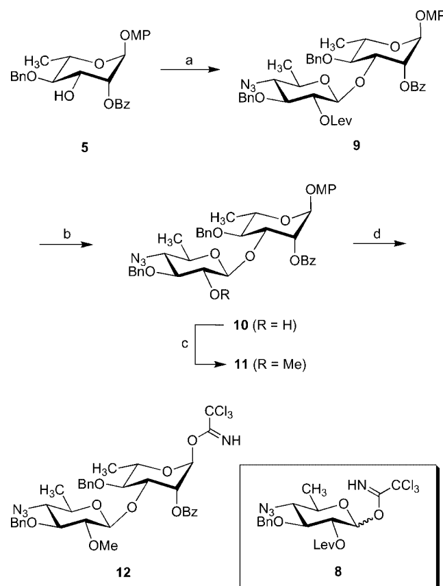
Scheme 2. Synthesis of disaccharide building block 12 . Reagents and conditions: a) 8 , TMSOTf, CH 2 Cl 2 , 0 °C, 1 h, 98%; b) N 2 H 4 ·AcOH, CH 2 Cl 2 /MeOH (5:1), 25 °C, 12 h, 83%; c) NaH, MeI, DMF, 1 h, 25 °C, 81%; d) 1) CAN, H 3 CCN/H 2 O (1:1), 25 °C, 85%, 2) Cl 3 CCN, CH 2 Cl 2 , NaH (cat.), 25 °C, 90%.
