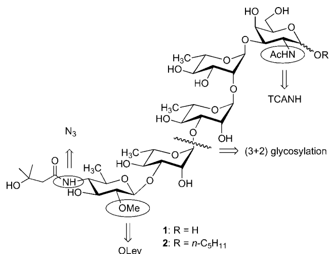
Figure 1. Structure of pentasaccharide 1 attached to the spore surface protein BclA of B. anthracis and analogue 2 that was synthesized.
