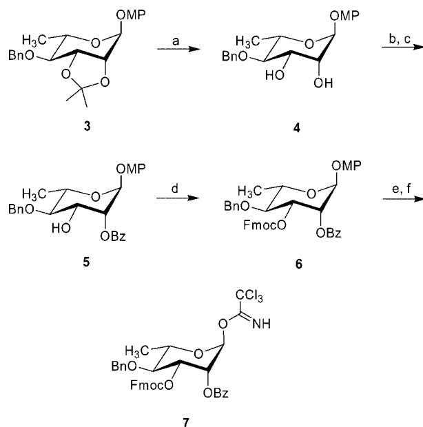
Scheme 1. Synthesis of rhamnose building block 7 . Reagents and conditions: a) HCl (pH 3), MeOH/H 2 O (10:1), 45 °C, 89%; b) PhC(OMe) 3 , CSA (cat.), CH 2 Cl 2 , 25 °C, 2 h; c) AcOH/H 2 O (4:1, v/v), 30 min, 90% (2 steps); d) FmocCl, pyridine, 25 °C, 2 h, 88%; e) CAN, H 2 O/CH 3 CN (1:1), 25 °C, 2 h, 86%; f) Cl 3 CCN, CH 2 Cl 2 , NaH (cat.), 25 °C, 2 h, 85%.
